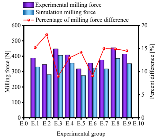
Fig. 11. Comparison of milling force experiments values and simulation values
