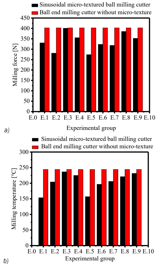
Fig. 5. Finite element simulation data image with parameter combinations obtained from nine sets of finite element simulation experiments; a) milling force variation, and b) variation of milling temperature
