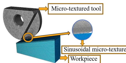
Fig. 4. Assembly model of tool-workpiece in finite element simulation
