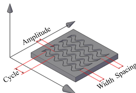
Fig. 3. A three-dimensional model of sinusoidal micro-texture
